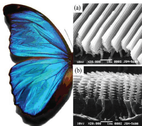
Figure 6. Left: Morpho menelaus . Image reproduced with permission under the terms of the GNU Free Documentation License [16]. Scanning electron microscopic images of the cross-sections of ground scales of M. rhetenor (Fig. 6a) and M. didius (Fig. 6b). Images reproduced with kind permission from The Royal Society [17].
