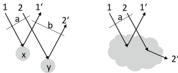
Figure 4. Coherent (left) and incoherent scattering (right).
