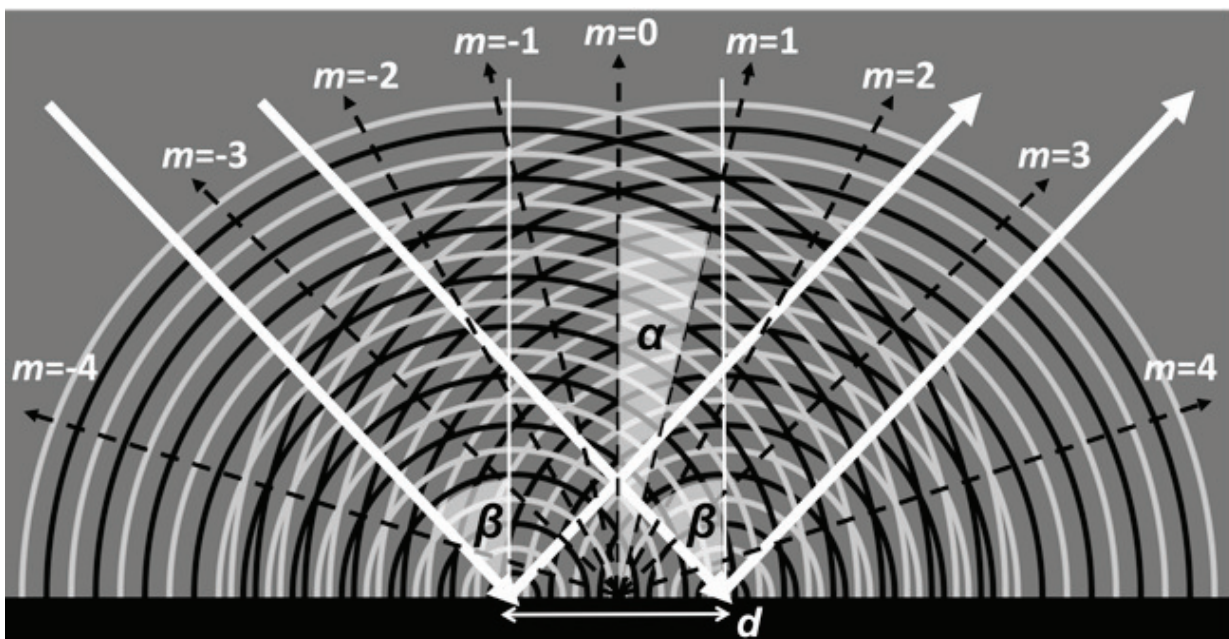
Figure 3. Colour production in a diffraction grating, represented by the black bar on the bottom.
