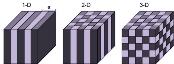
Figure 5. Schematics of one-, two- and three-dimensional photonic crystals (1-D, 2-D, 3-D). The colours represent materials with different refractive indices. The spatial period of the material is called the lattice constant, a .
