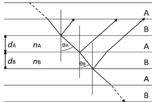
Figure 2 (right). Multilayer interference n_B > n_A . A change in viewing angle corresponds to a change in the perceived colour, due to changes in the phases of the interfering waves.
