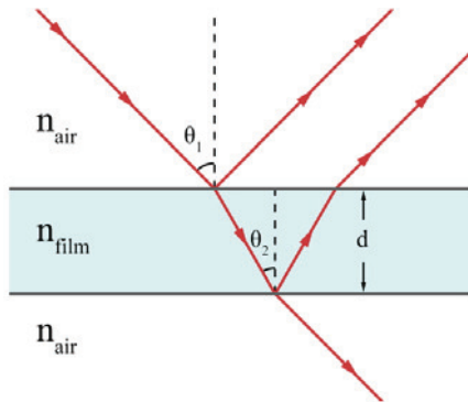
Figure 1. Thin film interference [13].
